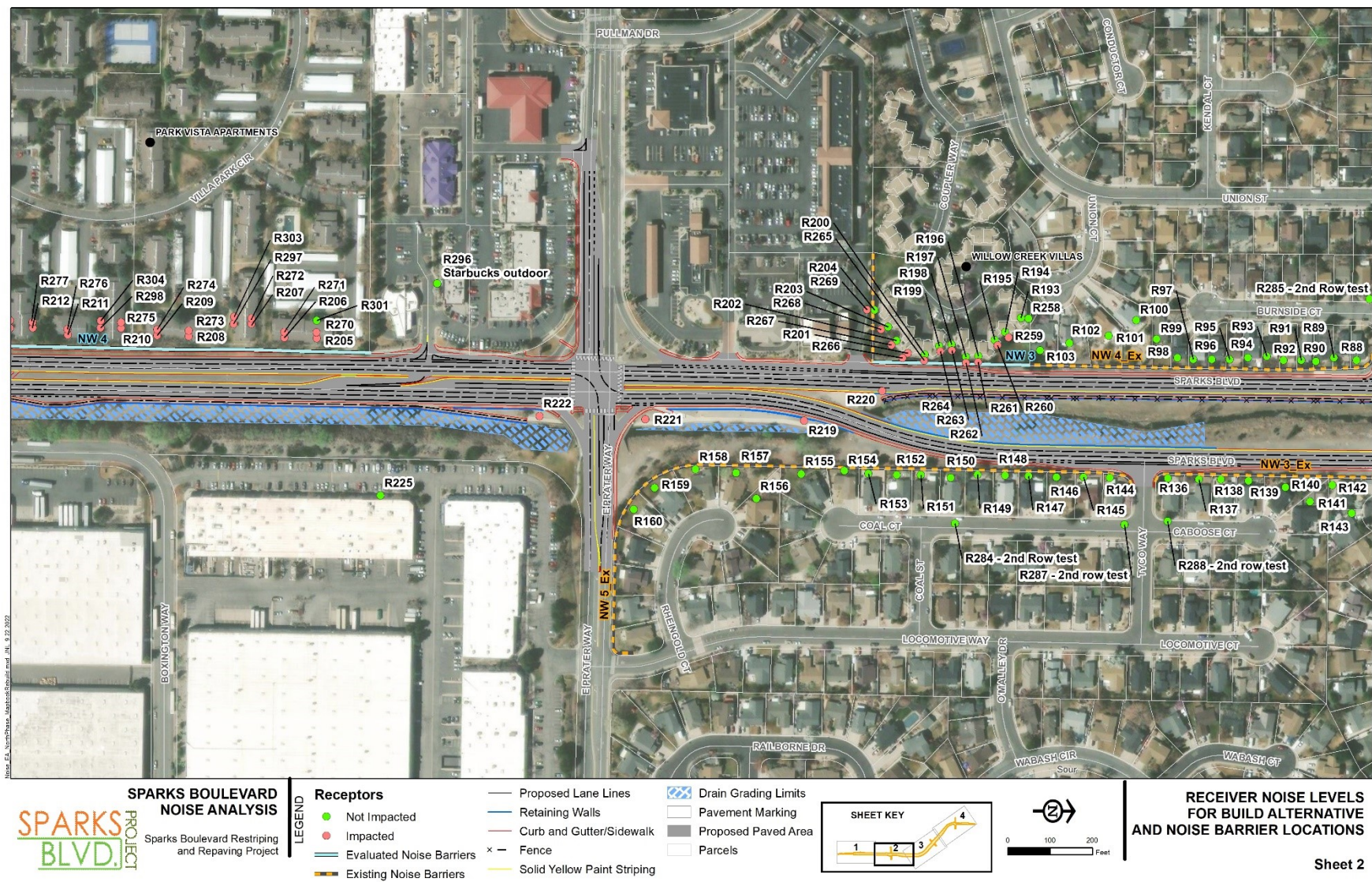
1 Figure 9. Traffic Noise Receptor and Barrier Locations (cont'd.)
